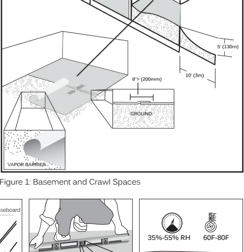
Figure 1: Basement and Crawl Spaces
